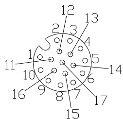
Pin Assignment
