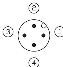
Pin Assignment
