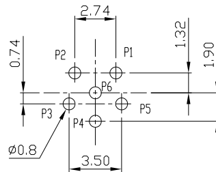
Recommend PCB Layout Component Side
