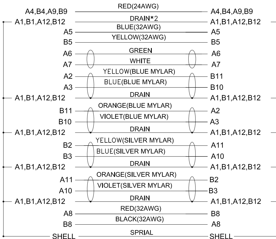
Wiring Diagram
