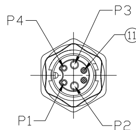
Pin Assignment
