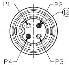
Pin Assignment
