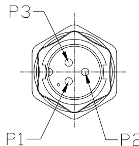
Pin Assignment
