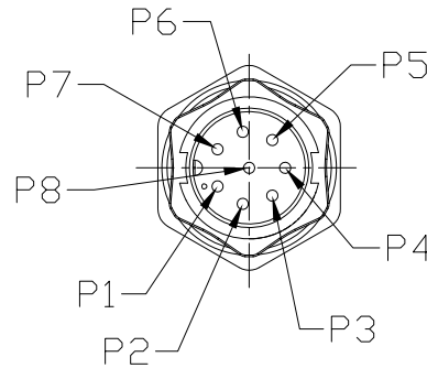
Pin Assignment
