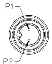
Pin Assignment
