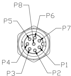
Pin Assignment
