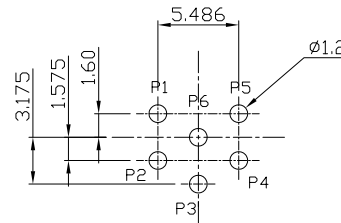
Recommend PCB Layout Scale 2:1
