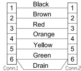
Wire Diagram
