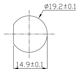
Recommend Panel Cut-Out
