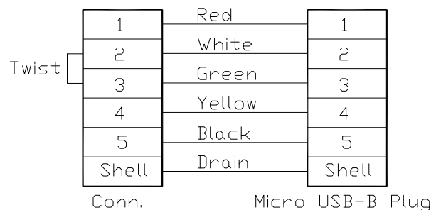
Wiring Diagram
