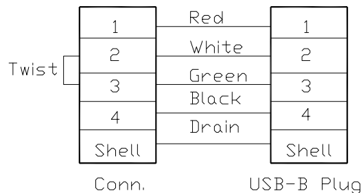
Wiring Diagram
