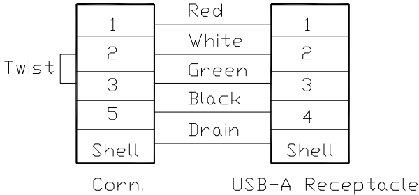
Wiring Diagram
