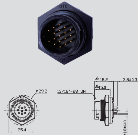
Plastic C3 Panel Mount Male Dip Lock
