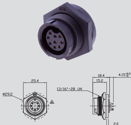
Plastic C3 Panel Mount Female Solder Lock
