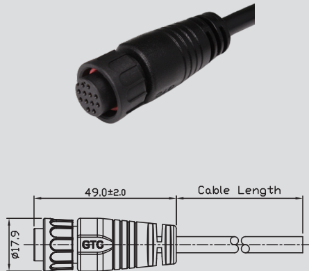
Plastic C2 Cable End Female Lock with Cable
