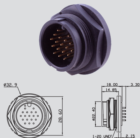
Plastic C4 Panel Mount Male Dip Lock
