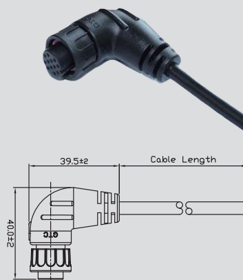
Plastic C2 Cable End 90° Key Down Female Lock with Cable
