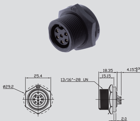
Plastic C3 Panel Mount Female Solder Screw
