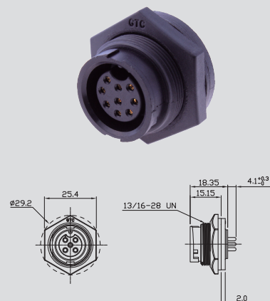
Plastic C3 Panel Mount Female Dip Lock
