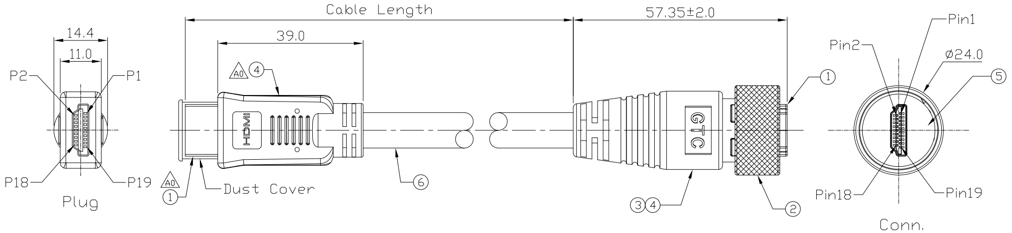
HDMI 19PIN MALE WITH PCB TYPE
