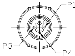
Pin Assignment
