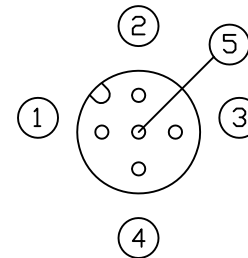
Pin Assignment Front View Scale 2:1
