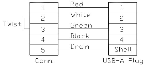
Wiring Diagram
