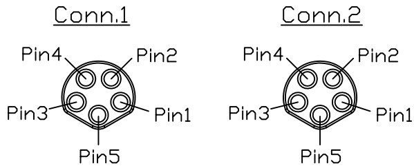
Pin Assignment
