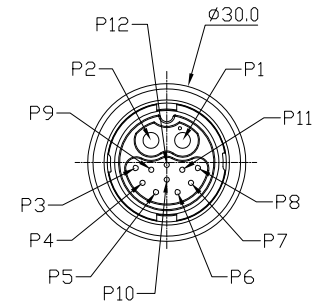
Conn.2
