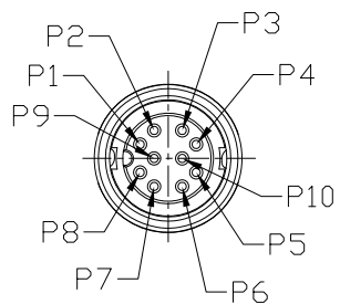
Conn.2
