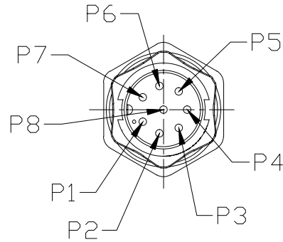
Pin Assignment
