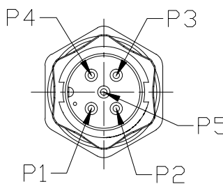
Pin Assignment
