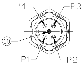
Pin Assignment
